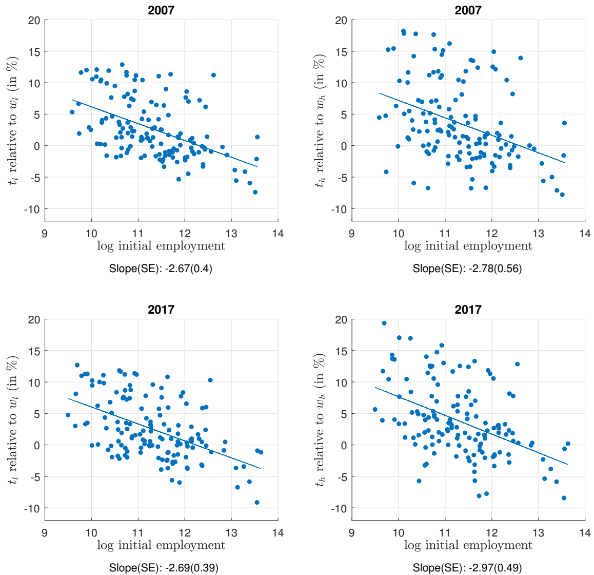
Figure 5: Optimal transfers
