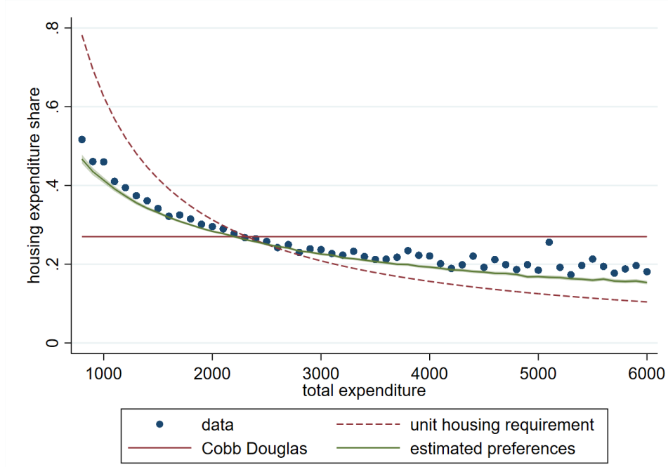
Figure 3: Preference calibration
