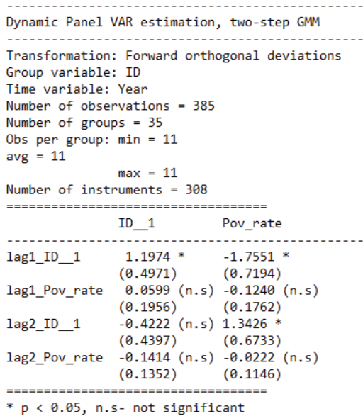
Figure 4. Vector autoregression model results for the analyzed data.
