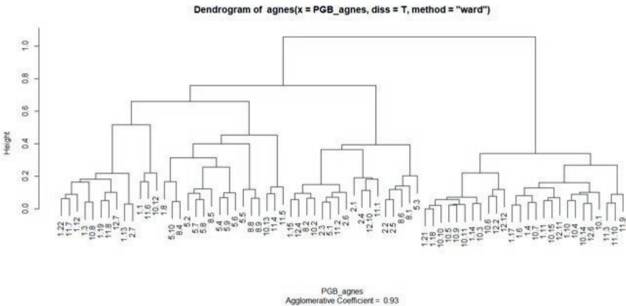
Cluster dendrogram.
