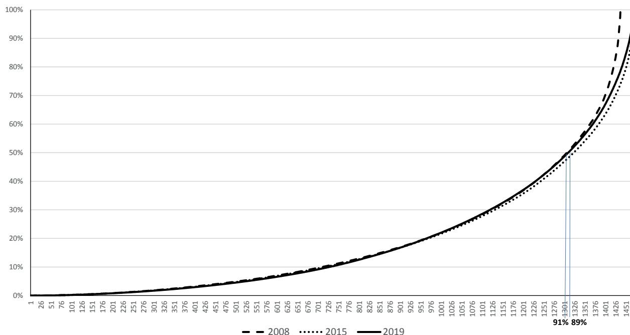
Figure A3. Lorentz curve of the (positive) farm net income within the Italian 2008-2019 FADN balanced sample: years 2008, 2015, 2019.
