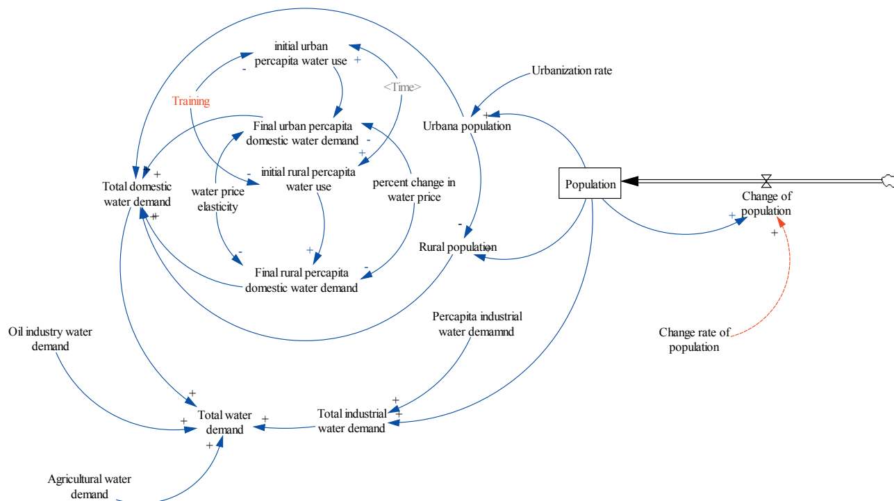
Figure 3. Population subsystem stock and flow diagram.
