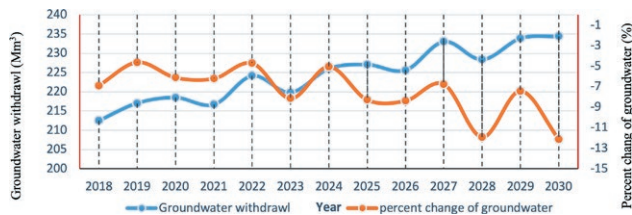
Figure 9. The result of simulated values of groundwater changes.
