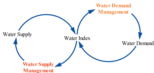
Figure 5. Interaction between water supply and demand.
