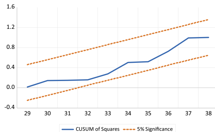
Figure 4. Cusum squares stability Test.
