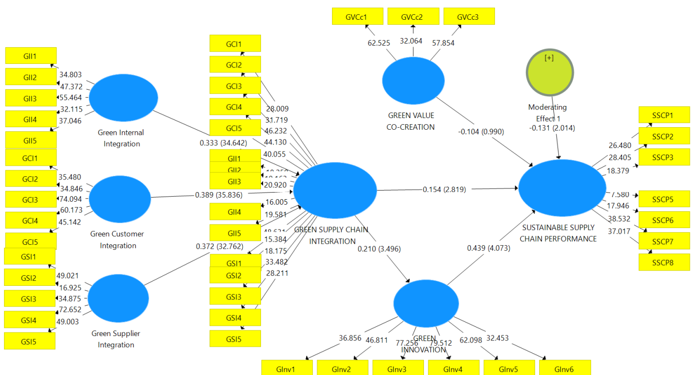
Figure 2. Path analysis.
