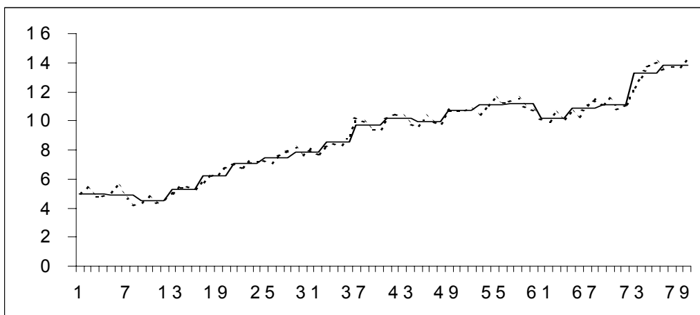
Fig. 3.1: Dividing by 4 1
