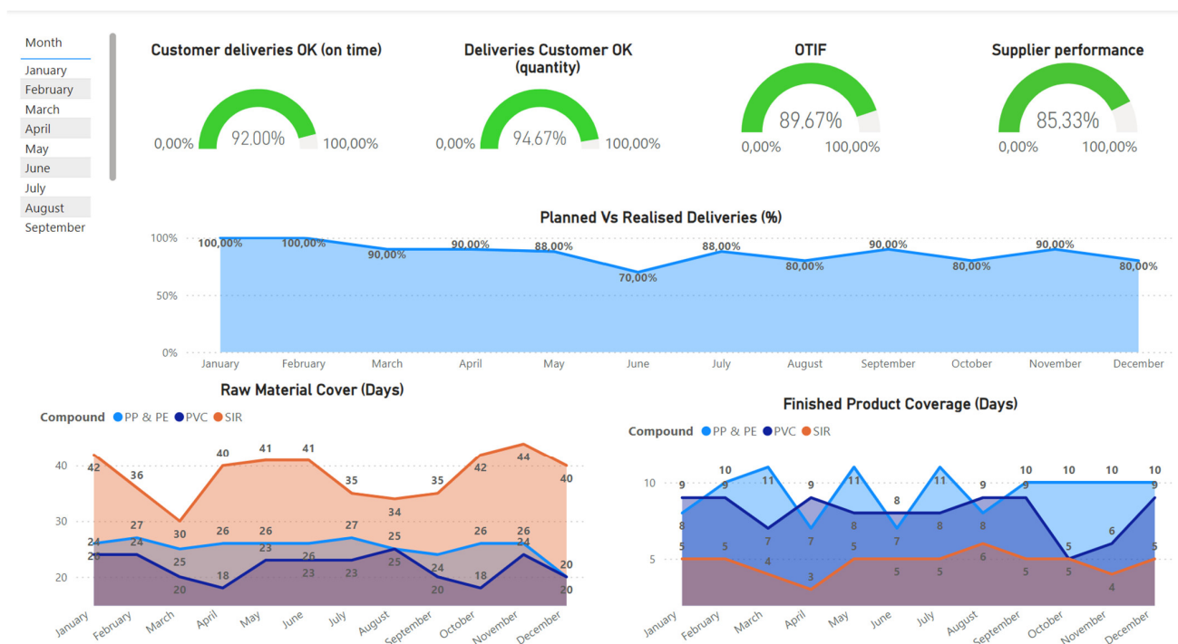
Figure 4. Dashboard developed for the Logistics department.
