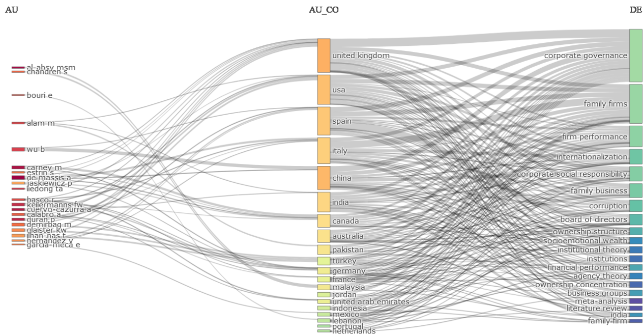
Figure 3. Sankey diagram.
