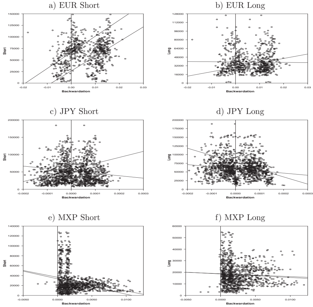
Figure 2: Short and long hedging and backwardation (continued): Strong backwardation is represented by ‘diamonds’ (◇) and weak backwardation is represented by ‘boxes’ (□).
