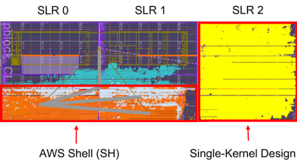
FIGURE 4. Single-kernel design: Resource utilization. Note: Resources utilized by: (i) the single-kernel CL design (yellow area); (ii) by the AWS shell (orange area); and (iii) available CL resources (other colors). The image is captured using Xilinx Vivado.
