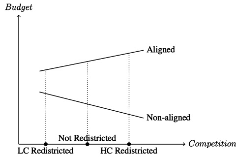
FIGURE 5. Theoretical predictions. Note. This figure outlines the main predictions of our model. Redistricting to a more competitive constituency will result in a larger (smaller) program scale in aligned (nonaligned) redistricted GPs, compared with non-redistricted GPs, thus resulting in a larger gap between the aligned and nonaligned GPs in this group. Within aligned GPs, those redistricted to more competitive constituencies will receive larger allocations than those redistricted to less competitive ones. The opposite will be the case for nonaligned GPs. In programmatic politics, these patterns will appear for both public and private programs, whereas in clientelism, they will appear only for private benefit programs.
