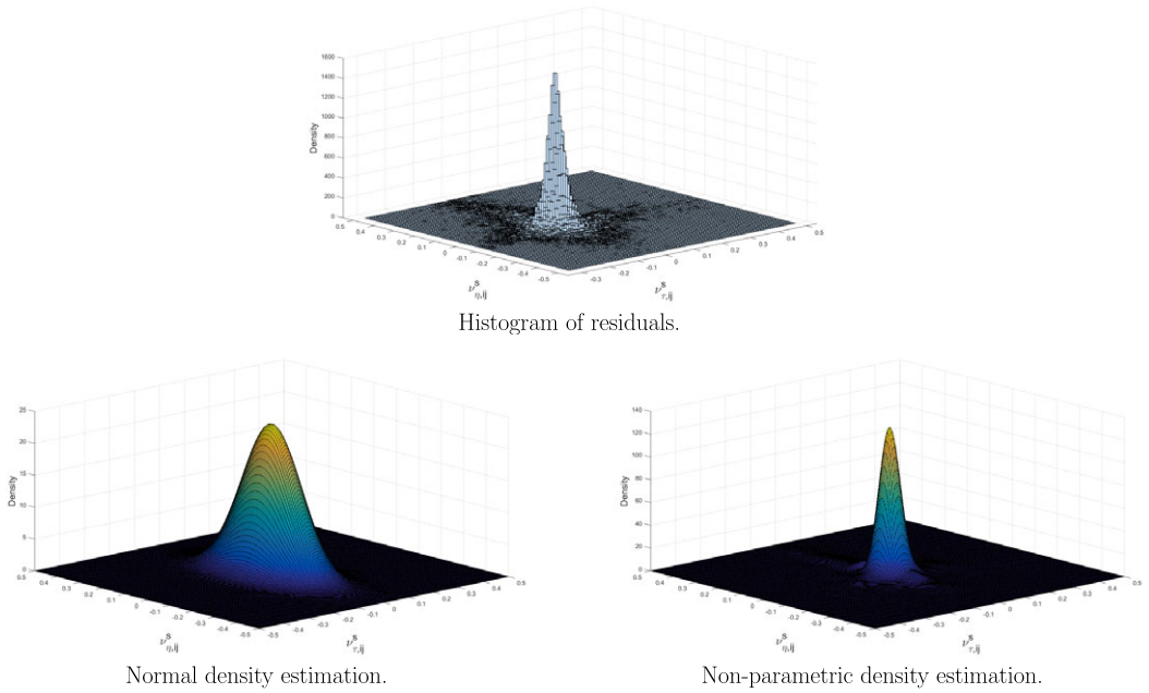
FIGURE S.2. Bivariate histogram of \nu_{ij}^s and its estimated distributions.
