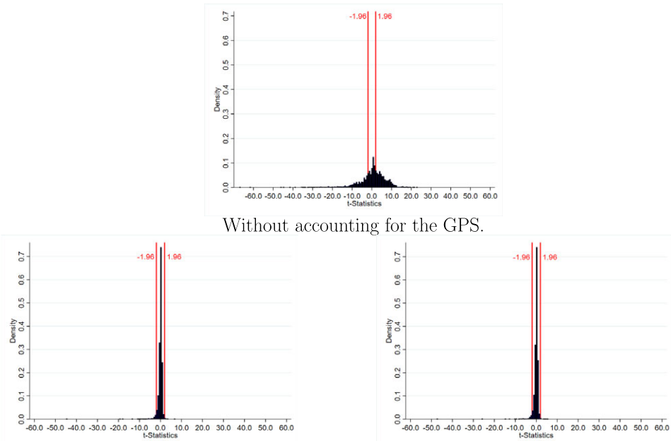
FIGURE S.3. Distribution of t -statistics of equality-of-means test for all covariates.
