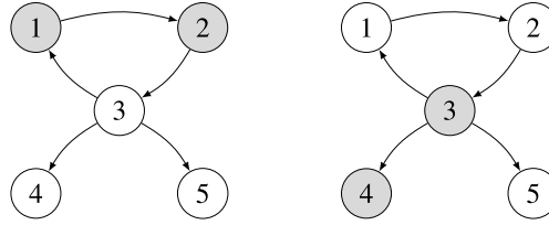
FIGURE 3. S = \{3, 4\} is more impactful than S' = \{1, 2\} .
