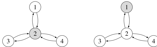
FIGURE 4. Seeds’ impact and Bonacich centrality.
