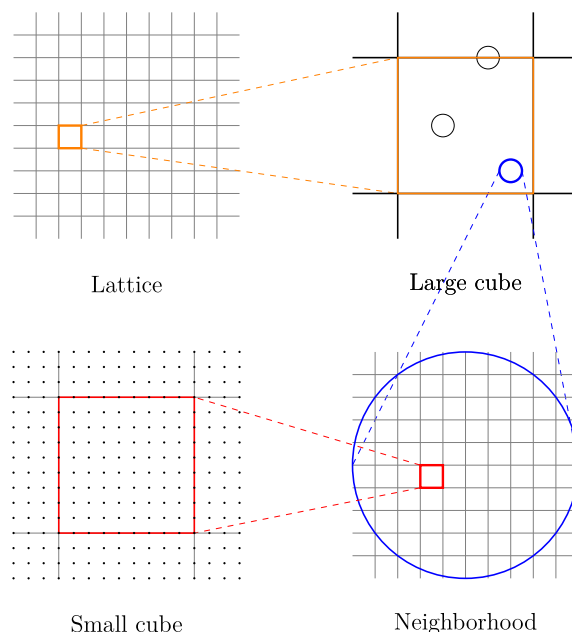
FIGURE 6. Lattice division.
