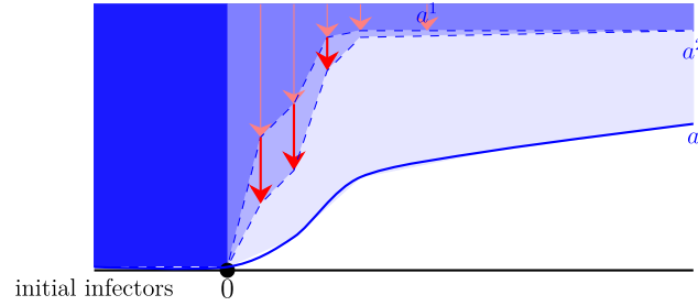
FIGURE 4. Contagion wave.
