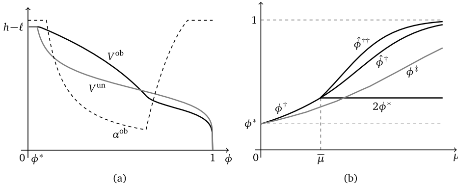
FIGURE 3. (a) V^{ob} and V^{un} for h = r = 1 , \ell = 0.05 , and \mu = 3 . (b) Thresholds for the public offers case ( \phi^\dagger , \hat{\phi}^\dagger , and \hat{\phi}^{\dagger\dagger} ) and the private offers case ( \hat{\phi}^\ddagger ) as a function of \mu , for h = r = 1 and \ell = 0.2 .
