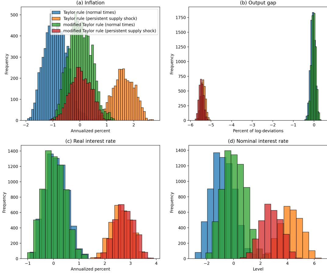
Figure 8: Ergodic distribution
