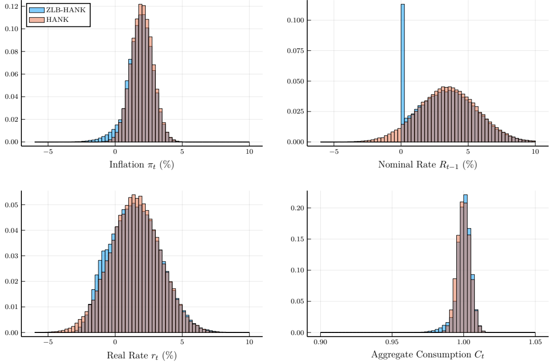
Figure 6: Ergodic Distributions
