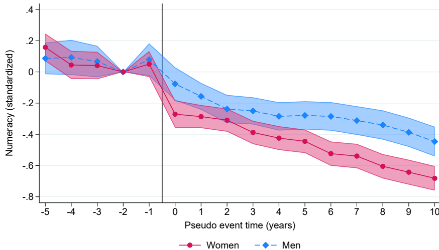
Figure 5: Child penalties in numeracy scores (without matching controls)
