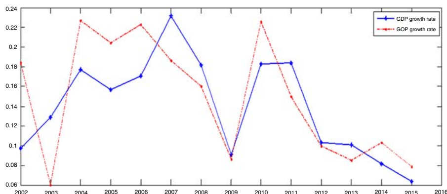
Figure 4. The growth rates of China GDP and GOP
