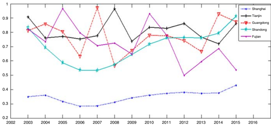
Figure 6. Temporal trends in GDP–GOP relational coefficients for the five provinces
