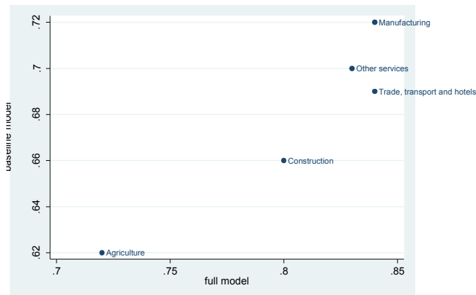
Figure 2 – Baseline model and full model AUC for each industry
