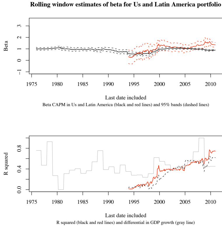
Figure 1: Rolling-Window Estimations(a)
