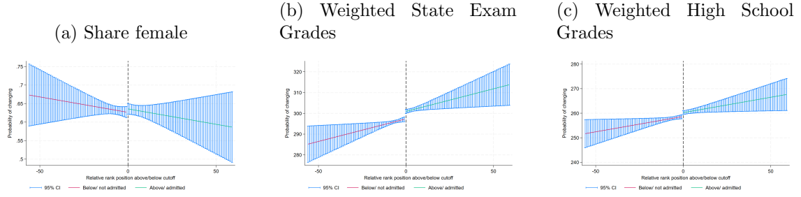
Figure A8: No discontinuity in counterfactuals, bw = 10%, 2012
