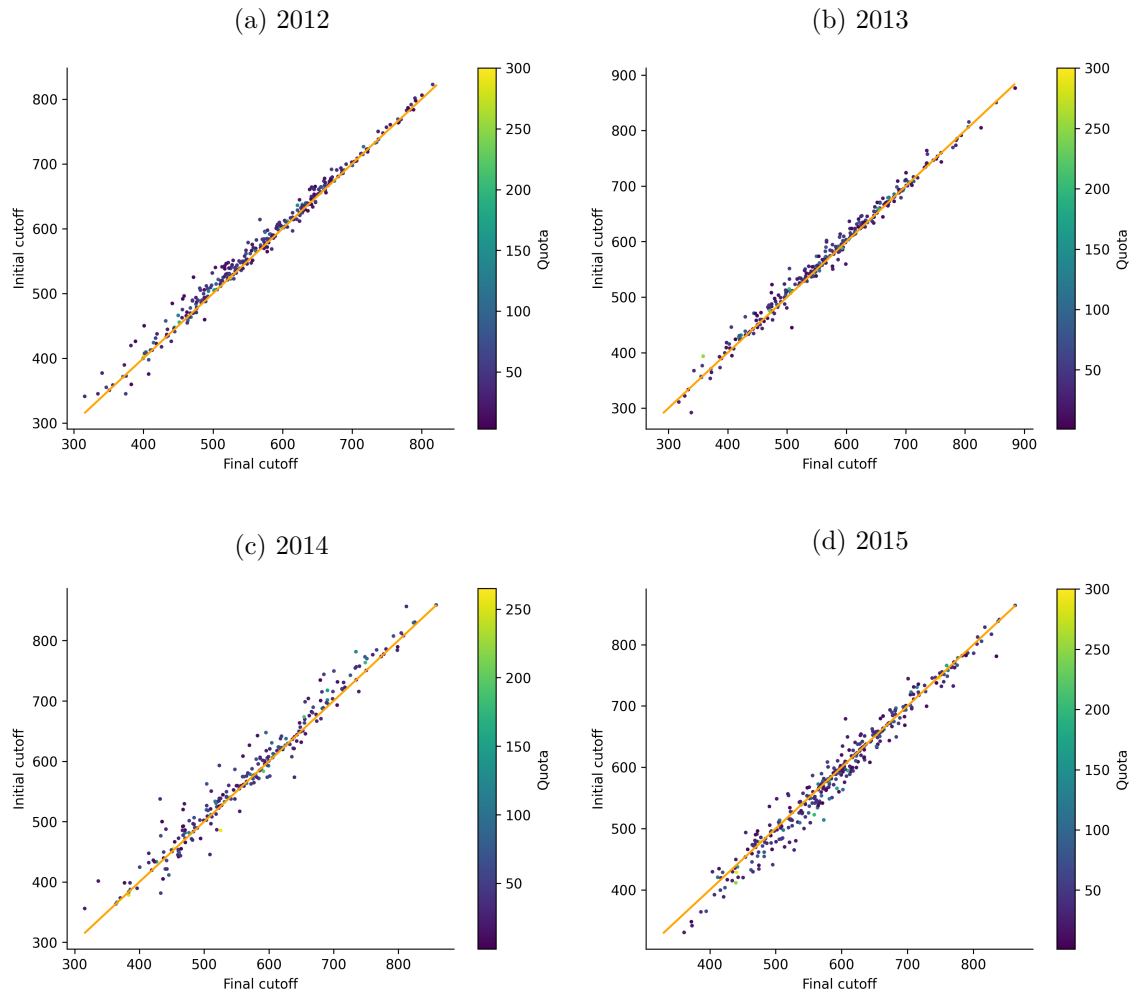
Figure A2: Initial and final cutoff scores
