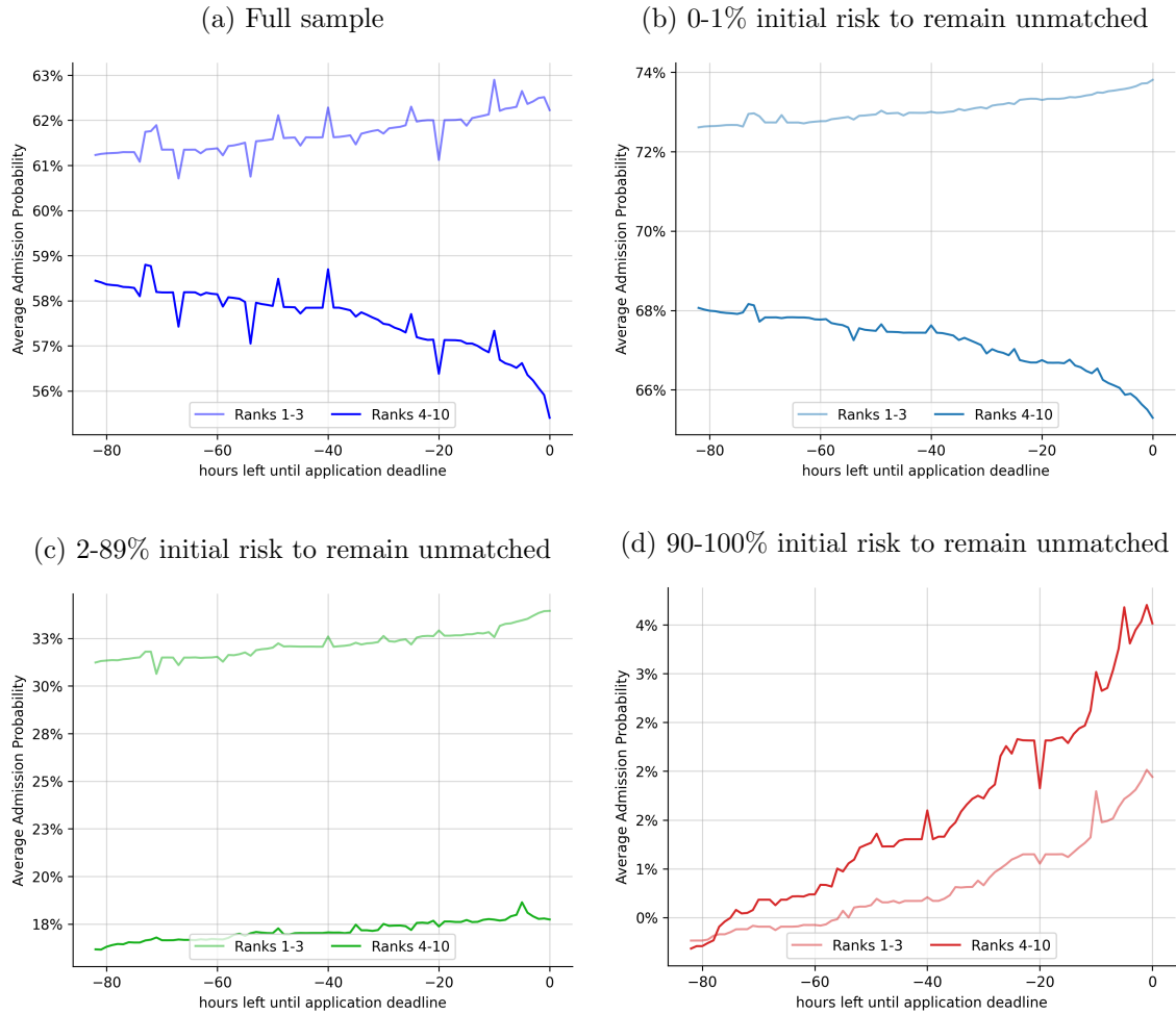
Figure A27: Average risk to remain unmatched over time, by initial risk (2012)
