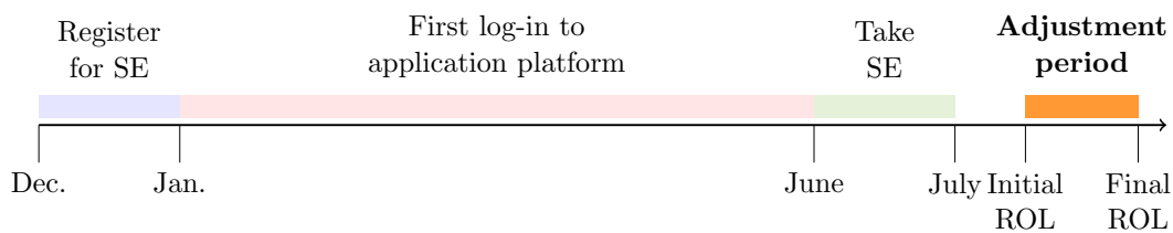
Figure 1: Timeline
