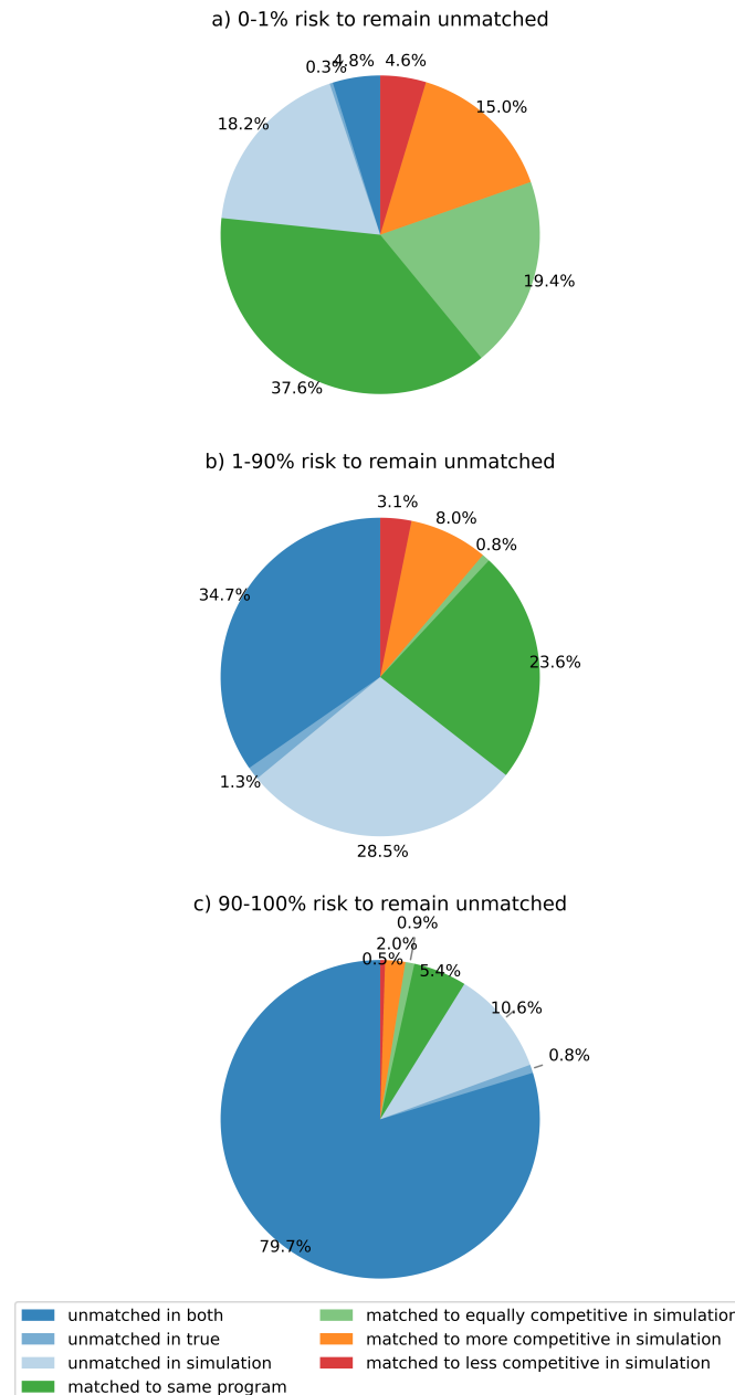
Figure 20: Admission outcome in the simulated vs. observed scenario, subgroups
