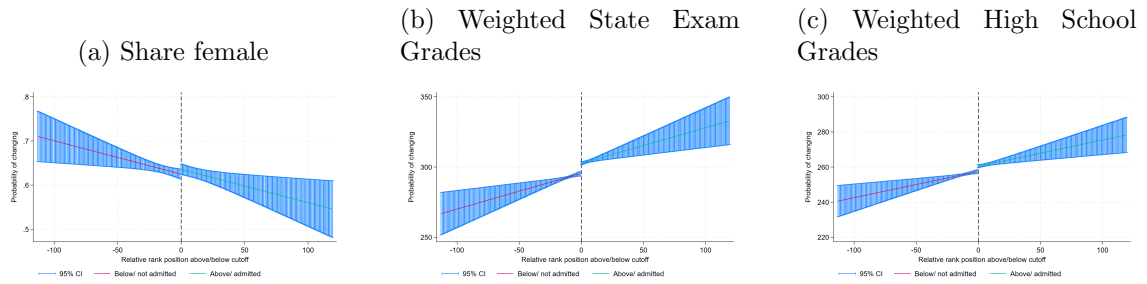
Figure A12: No discontinuity in counterfactuals, bw = 20%, 2012
