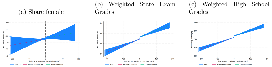
Figure A19: No discontinuity in counterfactuals, bw = 30%, 2015
