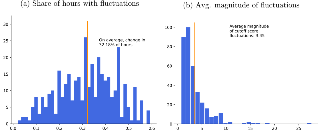
Figure 5: Distribution of programs by number and avg. magnitude of fluctuations
