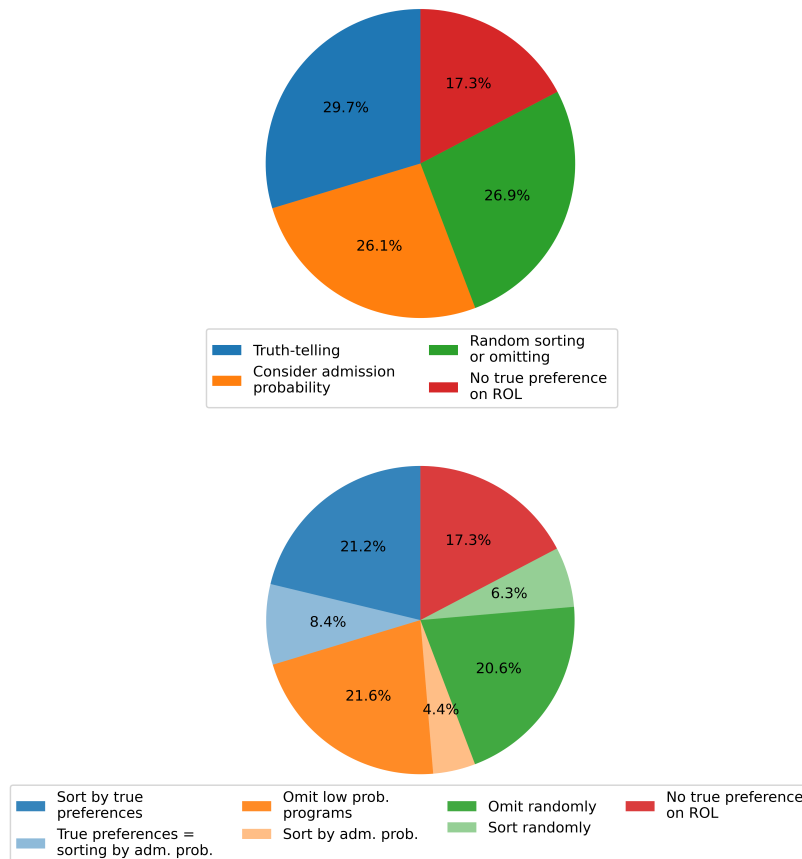
Figure 15: Strategic types
