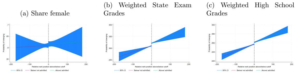
Figure A18: No discontinuity in counterfactuals, bw = 30%, 2014
