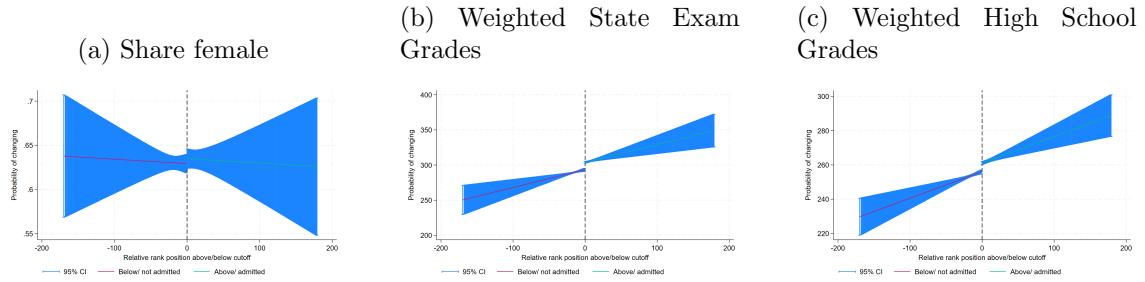
Figure A16: No discontinuity in counterfactuals, bw = 30%, 2012
