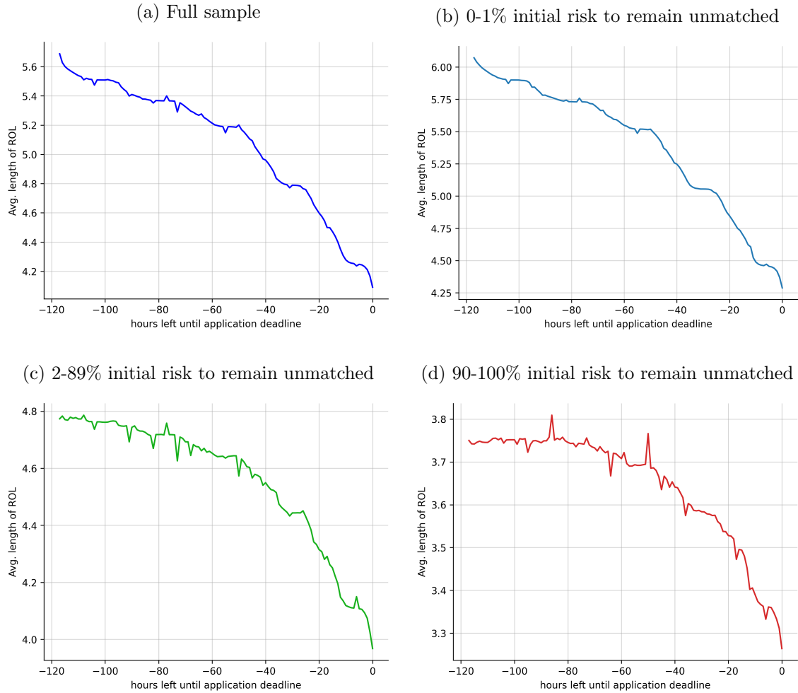
Figure A25: Average number of ranked programs over time, by initial risk (2013)
