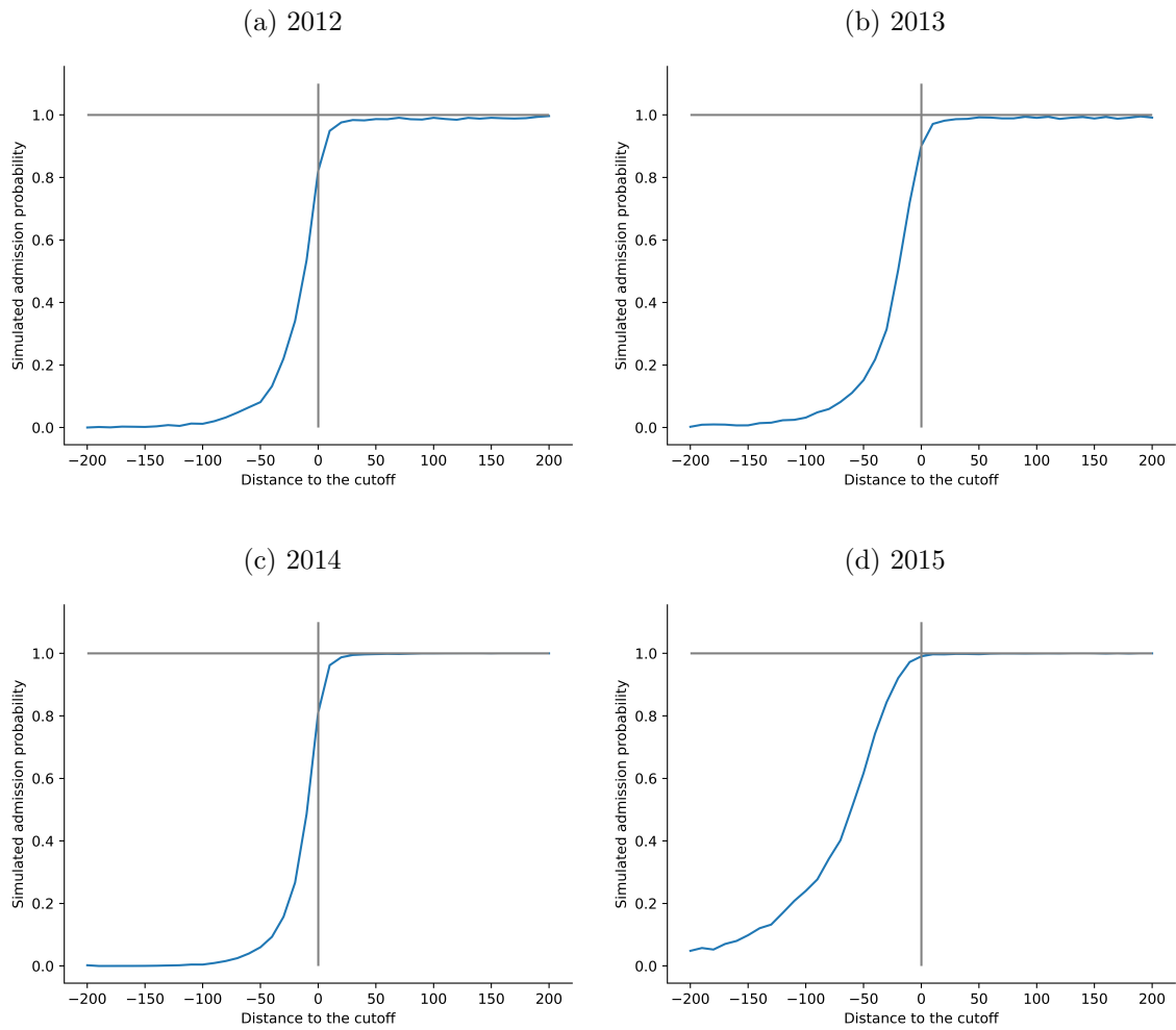
Figure A20: Simulated admission probability around the admission cutoff
