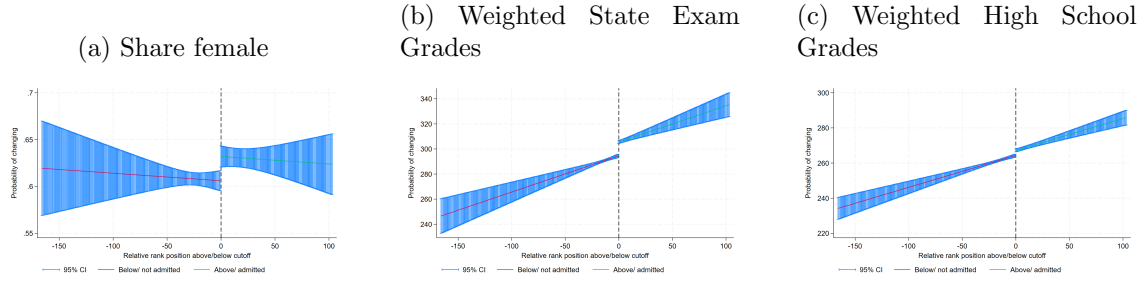
Figure A17: No discontinuity in counterfactuals, bw = 30%, 2013
