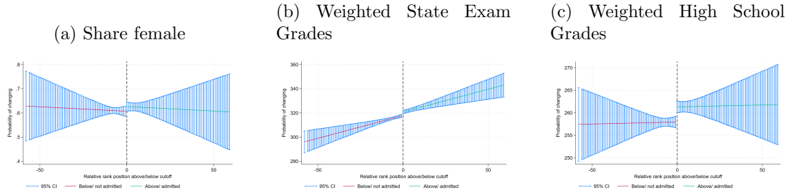
Figure A10: No discontinuity in counterfactuals, bw = 10%, 2014
