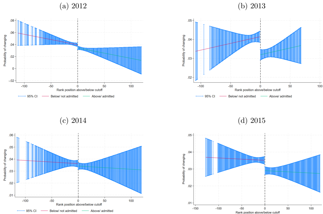
Figure A7: RDD, bw=20%, running variable = rank distance
