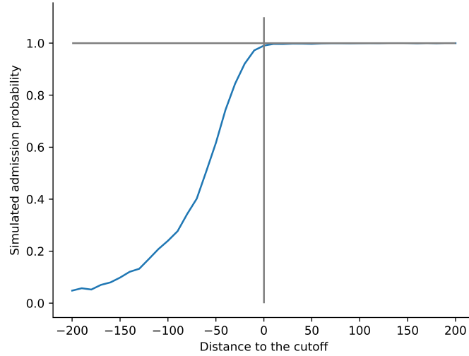
Figure 11: Simulated admission probability around the admission cutoff, 2015
