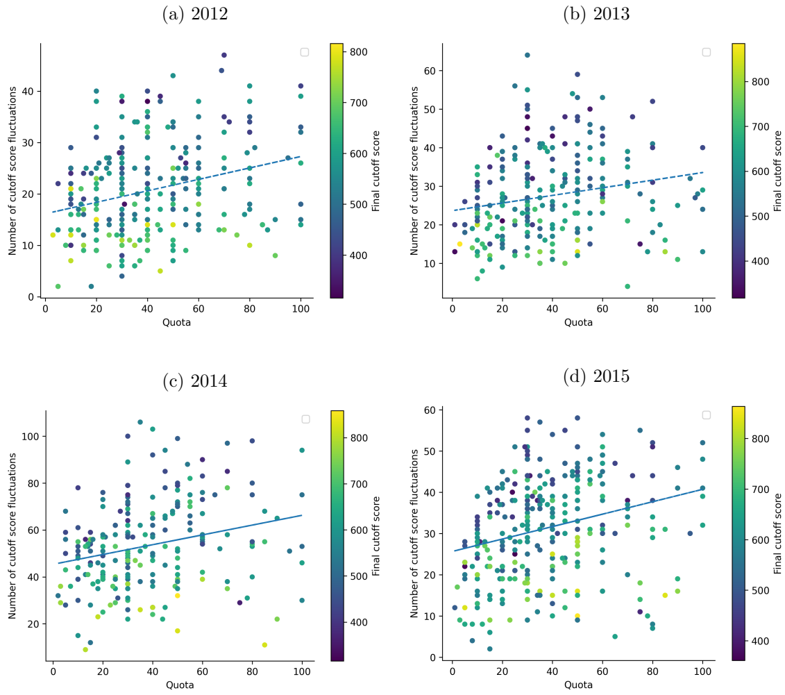
Figure A5: Number of fluctuations by program characteristics
