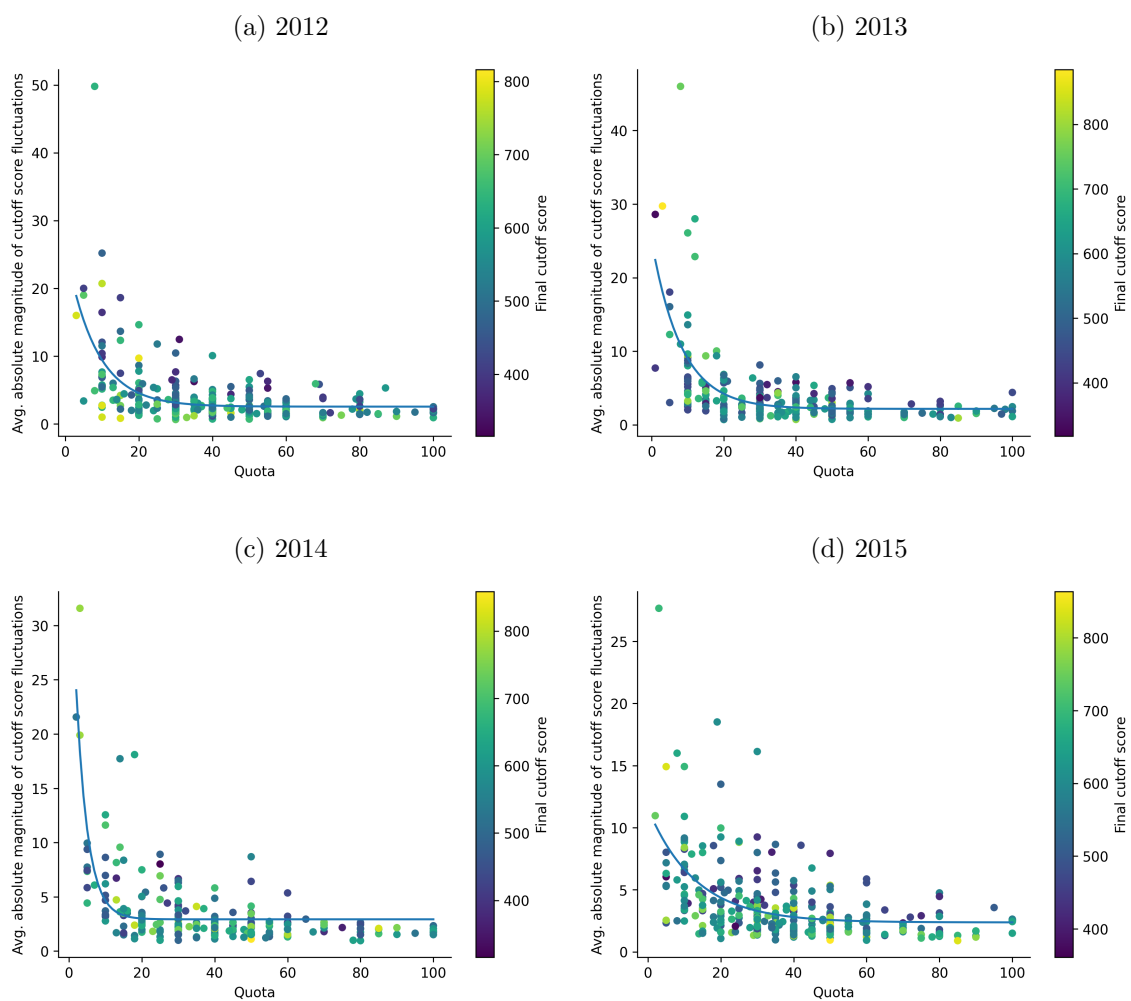
Figure A6: Magnitude of fluctuations by program characteristics
