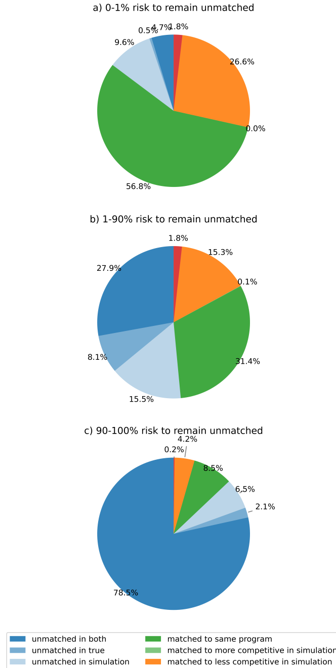
Figure 18: Admission outcome in the simulated vs. observed scenario, subgroups
