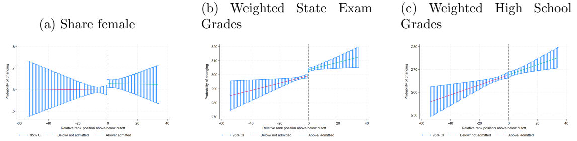
Figure A9: No discontinuity in counterfactuals, bw = 10%, 2013
