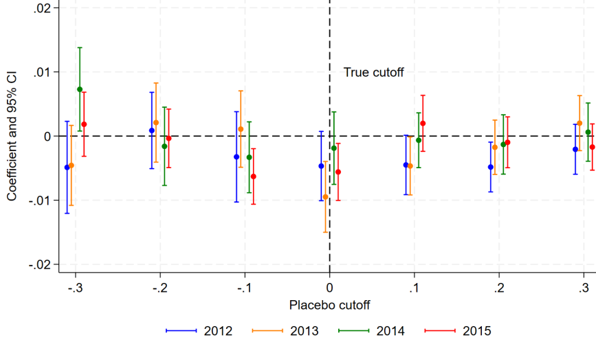
Figure 10: Coefficients with placebo cutoffs
