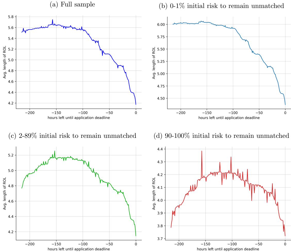
Figure A26: Average number of ranked programs over time, by initial risk (2014)
