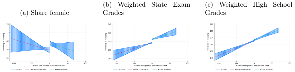
Figure A13: No discontinuity in counterfactuals, bw = 20%, 2013
