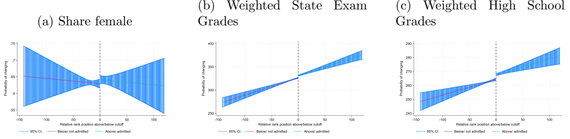
Figure 9: No discontinuity in counterfactuals, bw = 20%, 2015
