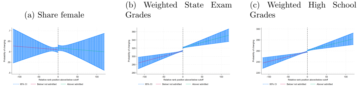
Figure A14: No discontinuity in counterfactuals, bw = 20%, 2014
