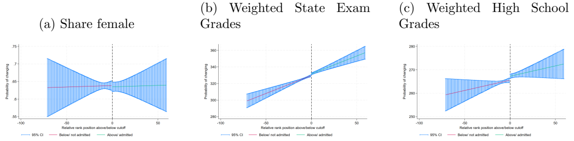
Figure A11: No discontinuity in counterfactuals, bw = 10%, 2015
