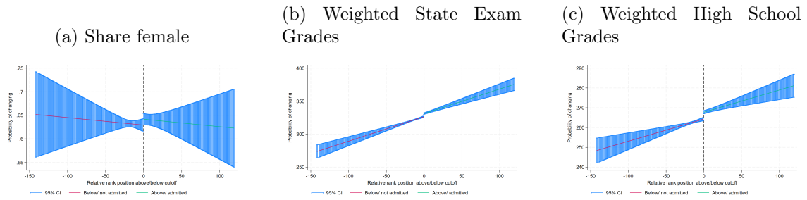
Figure A15: No discontinuity in counterfactuals, bw = 20%, 2015
