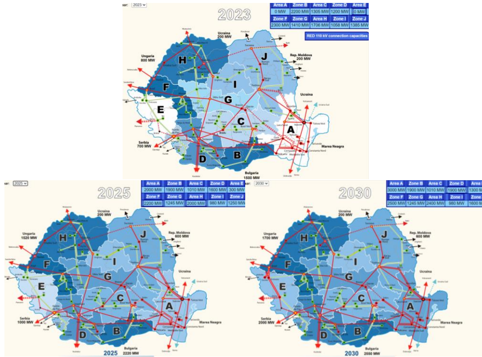
Figure 1. Available capacity to take over electricity production in the national grid Source: www.transelectrica.ro
