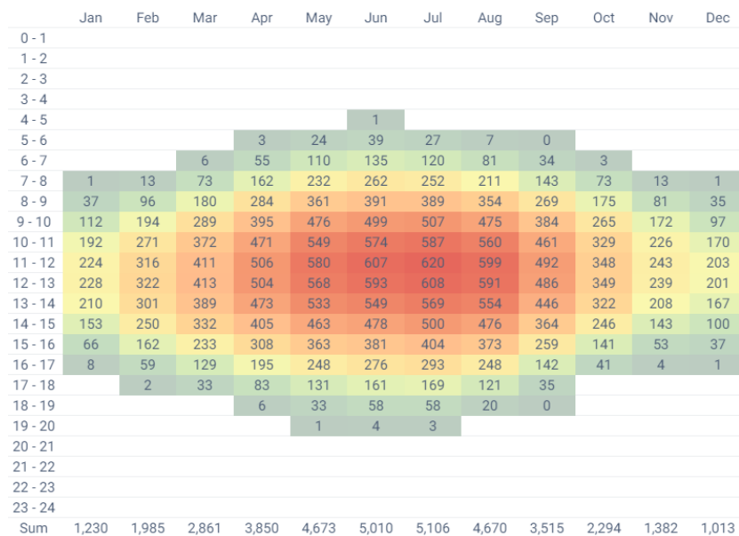
Figure 5. Average hourly photovoltaic power output
