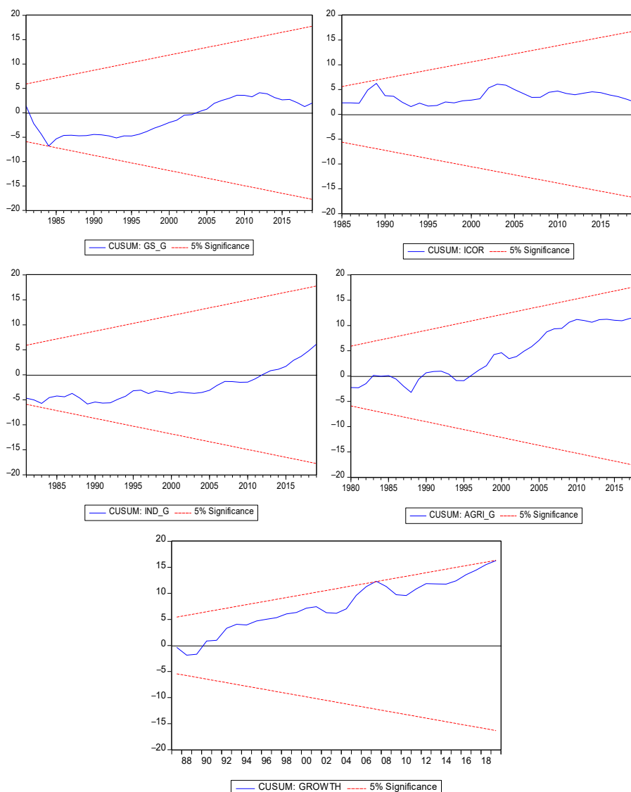
Figure 2. CUSUM test results
