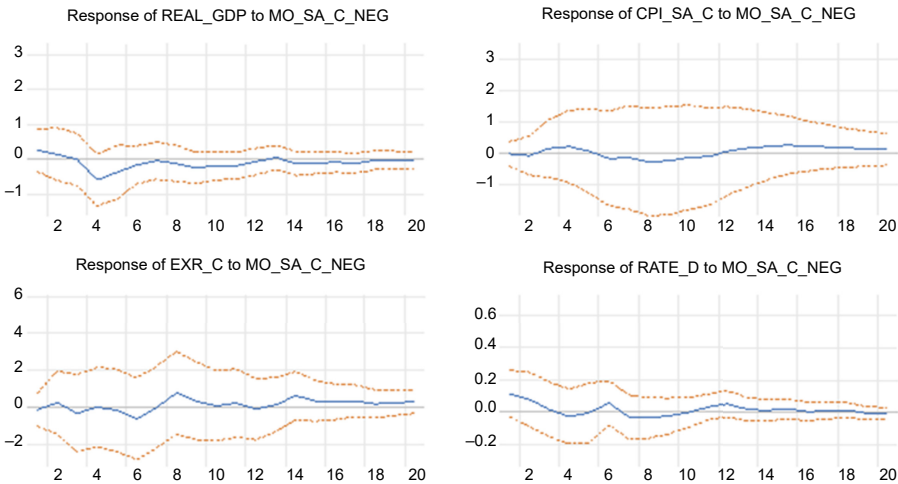
Figure 4. Impulse responses to negative M0 growth shocks <Asymmetric VAR> (data sample: 1996Q2–2018Q4)
