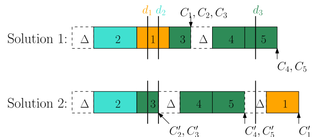
Fig. 1 An example for batch scheduling with 5 jobs. In Solution 1, jobs 1 and 5 are tardy. In Solution 2, only job 1 is tardy. Tardy jobs can be moved to the end of the schedule without increasing the weight of the tardy jobs
