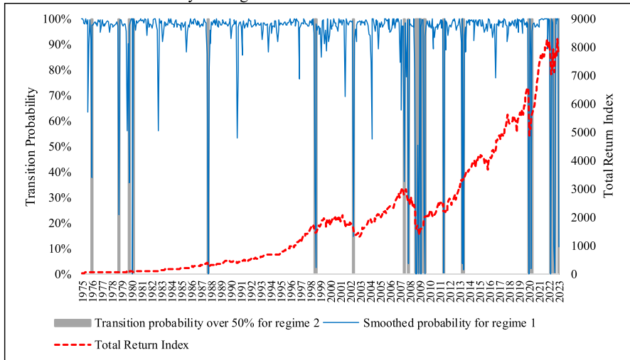
a. US Smoothed Probability of Regime 1
