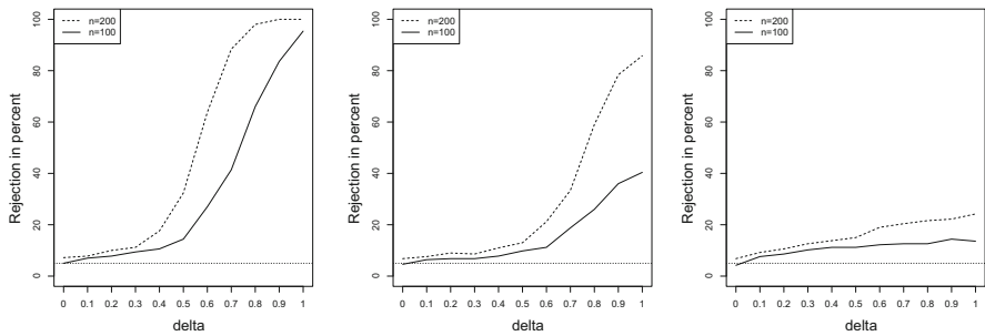
Fig. 1 Rejection probabilities with a change in the error distribution from \mathcal{N}(0, 1) to \tilde{F}_{1,\delta} (left), to \tilde{F}_{2,\delta} (middle) and to \tilde{F}_{3,\delta} (right). The dotted line marks the 5% level
