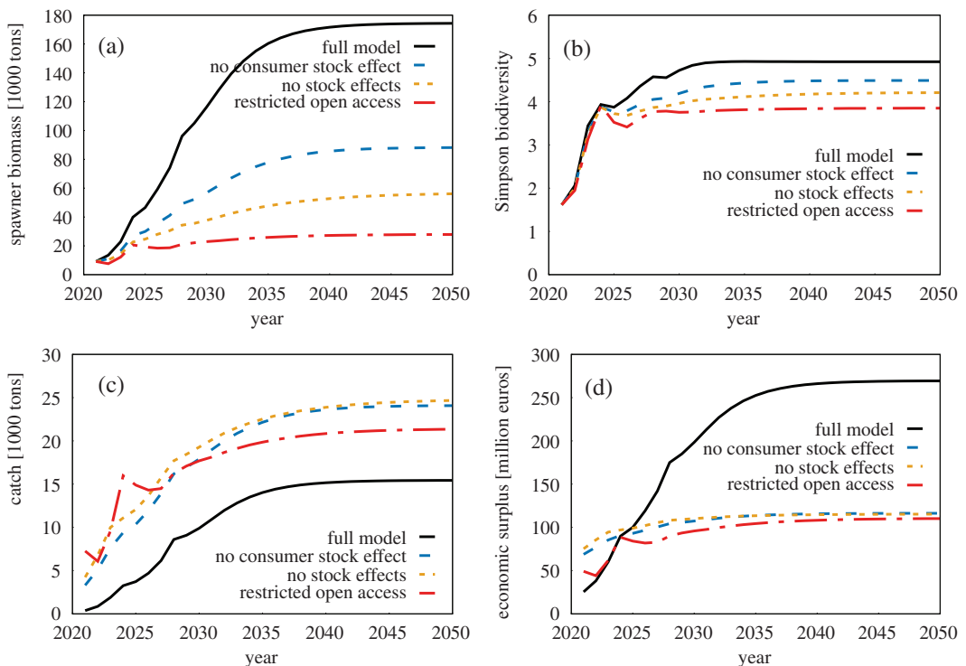
FIGURE 7 Time path of spawning stock biomass (a), Simpson biodiversity index (b), catch (c), and economic surplus (d) for different model configurations.
