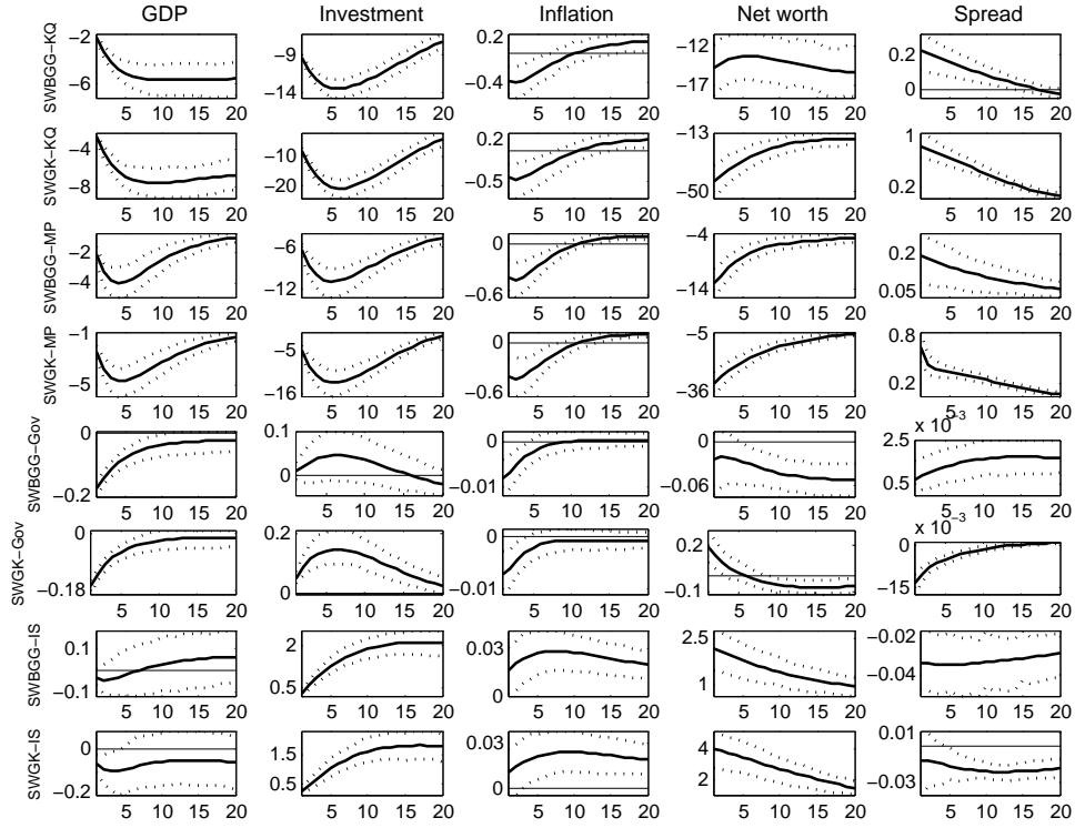
Figure 3: EA estimated impulse responses to the following shocks: capital quality (KQ), monetary policy (MP), government spending (Gov), and investment-specific technology (IS) in the SWBGG and SWGK models. Solid lines represent mean IRF and dashed line represent the 95% confidence intervals. The size of the shocks is normalized to one standard deviation.
