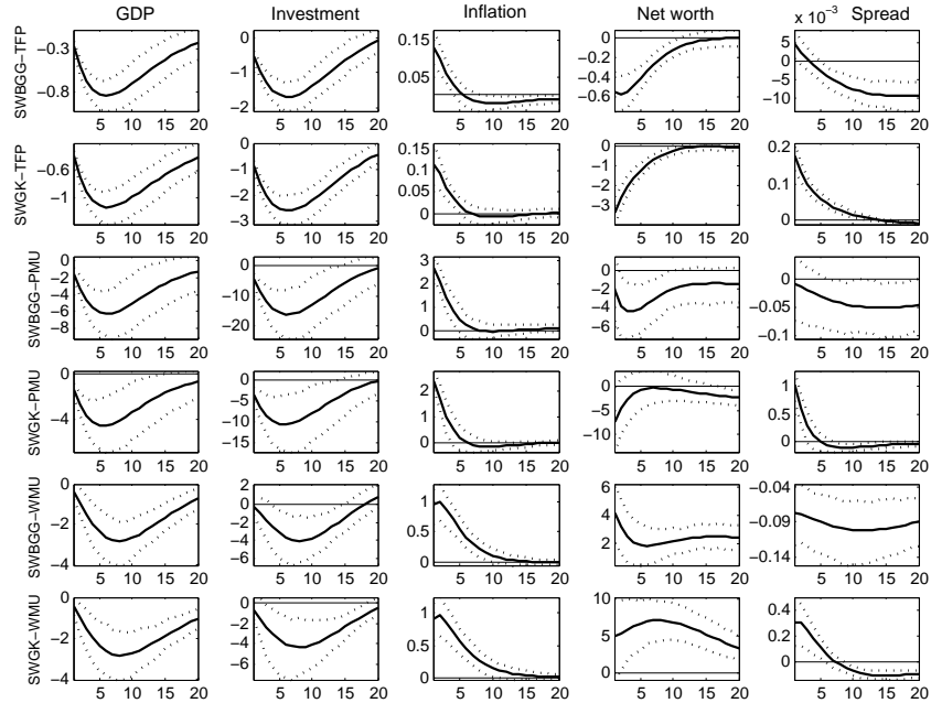
Figure 4: EA estimated impulse responses to the following shocks: TFP, price mark-up (PMU) and wage mark-up (WMU) in the SWBGG and SWGK models. Solid lines represent mean IRF and dashed line represent the 95% confidence intervals. The size of the shocks is normalized to one standard deviation.
