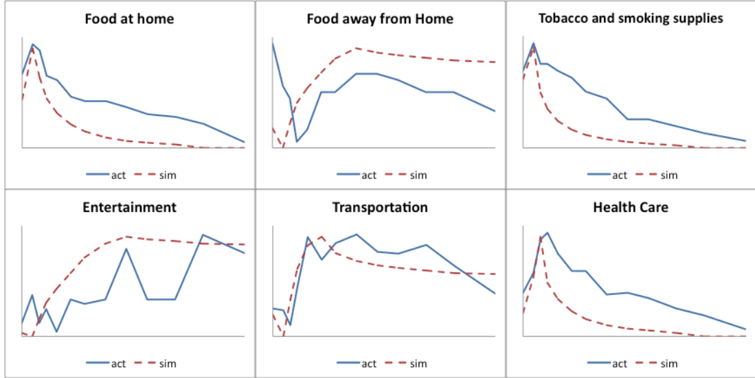
Figure 3. Simulated vs. observed Engel curves.
