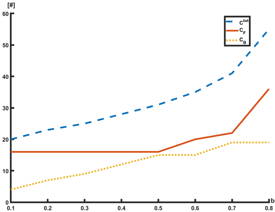
Fig. 6 Impact of b on the minimum number of agents C^{\text{tot}} and on the allocation
