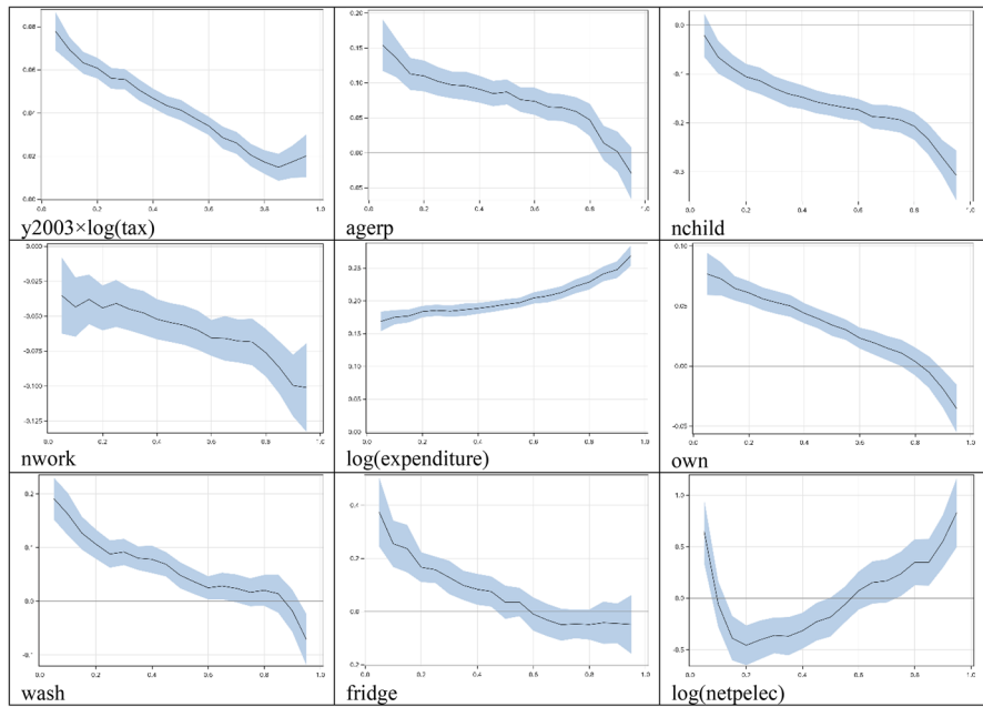
Fig. 6 Estimated quantile regression effect on electricity consumption p.p. with 95% confidence limits. x quantile levels; y regression coefficient of the respective variable
