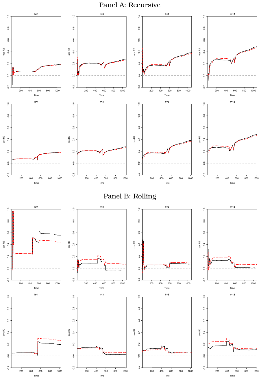
Fig. 2 Stability of results (gold). Note The figure plots the recursively estimated out-of-sample R^2 statistics for a training window (rolling-window) of length 60 (120) observations in the upper (lower) rows of Panels A and B. The first 120 out-of-sample forecasts are used to initialize the estimations. The solid black line shows the results for the combination AR/AR + GPC (RF). The dashed red line shows the results for the combination AR + share/AR + GPC (RF). (Color figure online)
