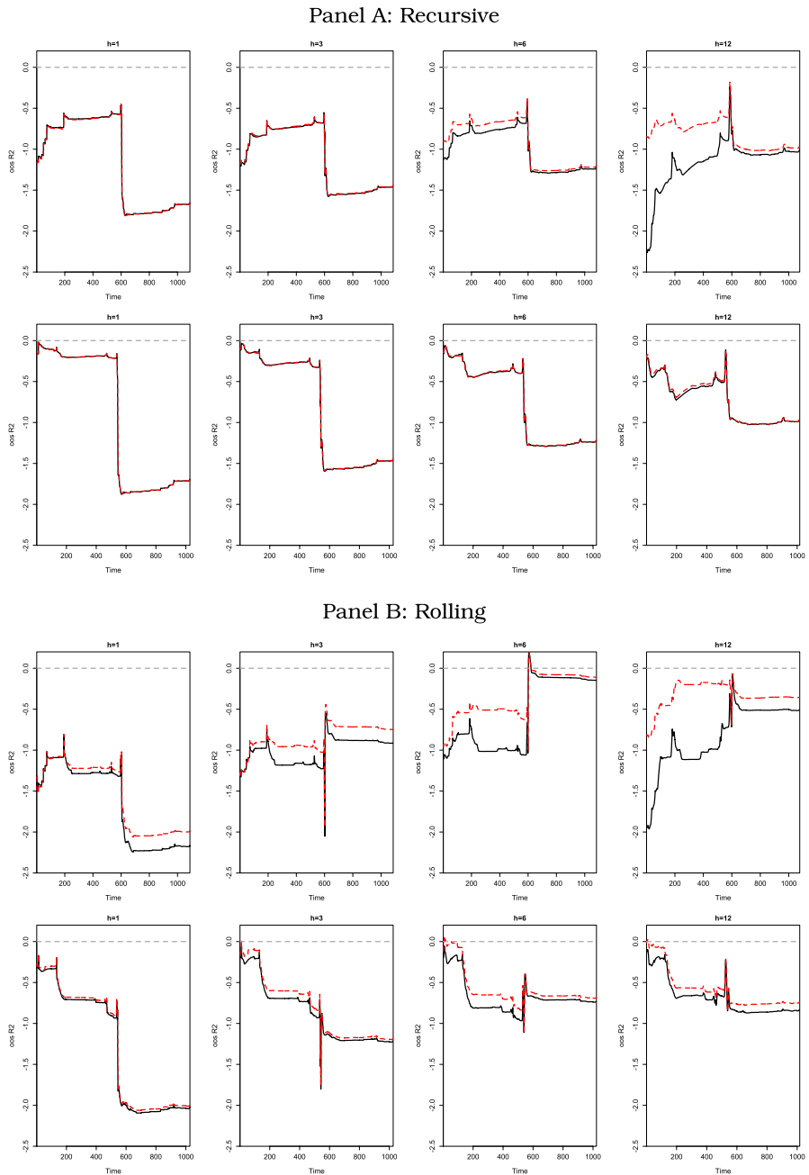
Fig. 4 Results for the out-of-sample R^2 statistic (Silver). Note: The figure plots the recursively estimated out-of-sample R^2 statistics for a training window (rolling-window) of length 60 (120) observations in the upper (lower) rows of Panels A and B. The first 120 out-of-sample forecasts are used to initialize the estimations. The solid black line shows the results for the combination AR/AR + GPC (RF). The dashed red line shows the results for the combination AR + share/AR + GPC (RF). (Color figure online)
