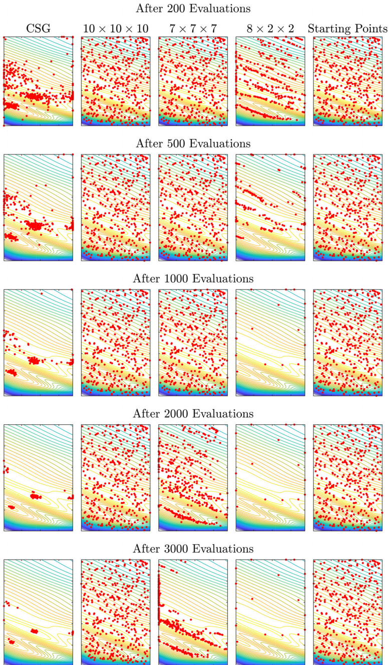
Fig. 9 Iterates of the different optimization approaches for (1) in the whole design domain \mathcal{U} = [1, 75] \times [1, 250] . For fmincon , the discretization of \Lambda \times \mathcal{R} \times \mathcal{D} is given in the titles, respectively. To measure the progress, the starting points are also shown. As mentioned above, an evaluation corresponds to the calculation of \text{Abs} , \text{Sca} , \text{Geo} , \nabla \text{Abs} , \nabla \text{Sca} and \nabla \text{Geo} for one combination (\lambda, \bar{R}, \bar{d}) \in \Lambda \times \mathcal{R} \times \mathcal{D} . Again, the underlying contours are obtained by discretizing \Lambda \times \mathcal{R} \times \mathcal{R} into 50 \times 50 \times 50 points
