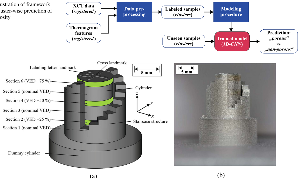
Fig. 2 Component design inspired by a study by Gobert et al. (2018) as computer-aided design (a) and after manufacturing (b). The specimen was manufactured from AISI 316L stainless steel. The outer staircase and the landmarks positioned on the specimen top were utilized for registration purposes (Oster et al., 2022). In the green component section
