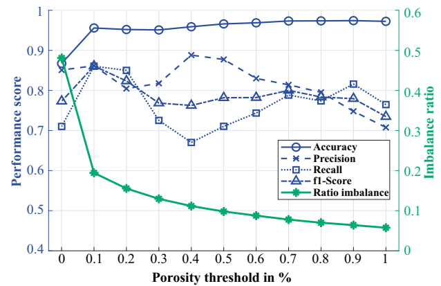
Fig. 9 Model performance depending on the set porosity threshold and imbalance ratio between both classes for a cluster dimension of (700 \times 700 \times 50) \mu\text{m}^3 and nine included subsequent layers
