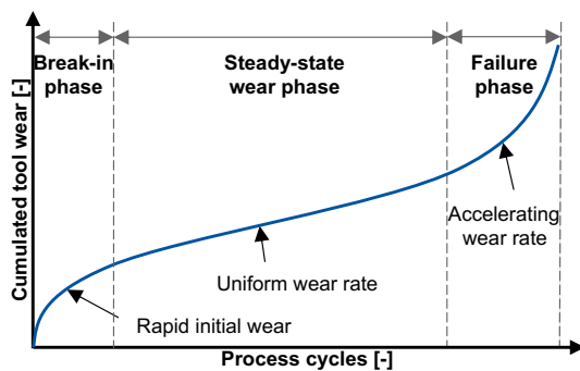
Fig. 1 Theoretical tool wear over the tool life
