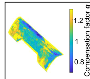
Fig. 5 Experimentally obtained local compensation factors g , which reflect the non-linear behaviour of the specific geometry at hand to linear compensation
