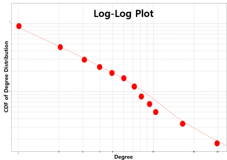
Figure 4. Cumulative degree distributions
