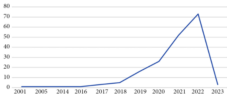
Figure 2. Publication trend
