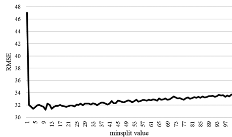
Figure 16. Model RMSE vs. minsplit value
