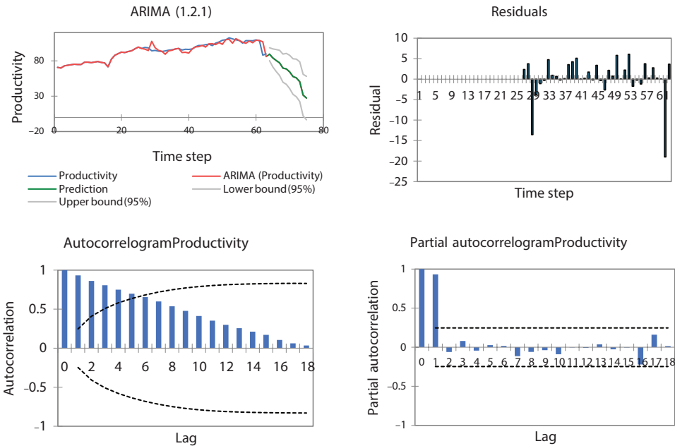
Figure 7. Detailed graphs for ARIMA (1,2,1) for Turkey
