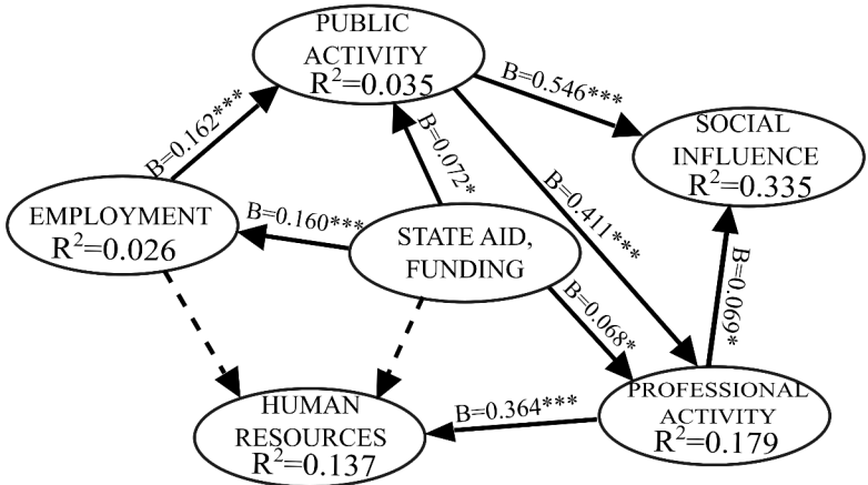
Figure 2. Final Path model and path coefficient estimates
