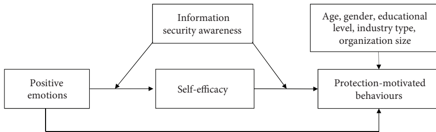
Figure 1. Research model
