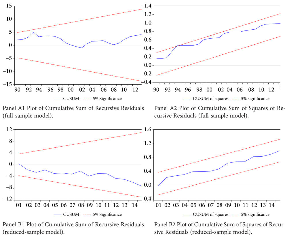
Figure 2. Stability tests for the ARDL models
