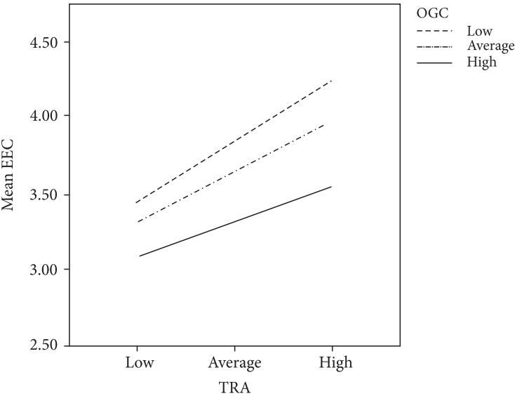
Figure 2. The conditional effect in OGC
