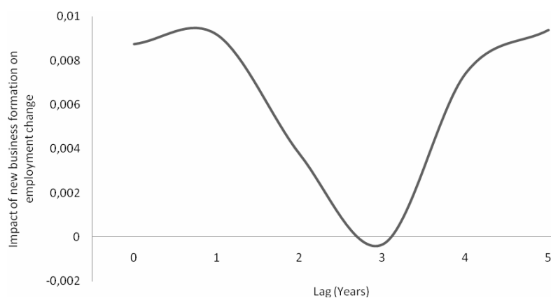
Figure 1. Estimated impact of total start-up rates on private employment change. The figure is based on estimated parameters of start-up rates with different lag lengths (see Equation 1).
