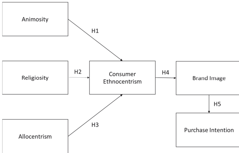
FIGURE 1. Theoretical framework
