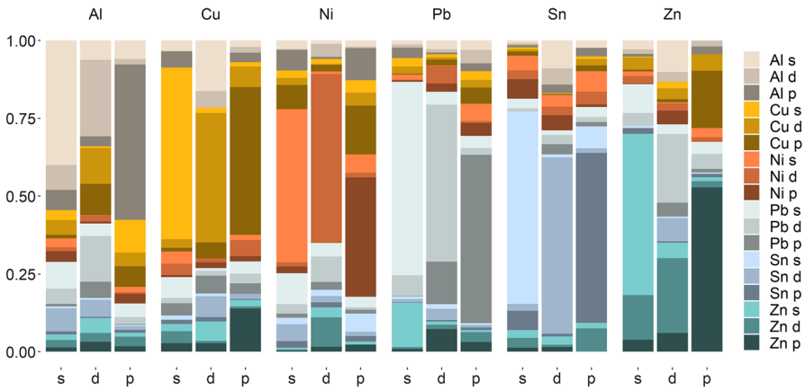
Fig. 2 Aggregated GFEVD plots for weight matrix demand ( D ). Scaled and aggregated GFEVD of the GVAR with weight matrix demand by the mean of 1 to 10 steps ahead per attribute, decomposed by the shocks of each endogenous variable
