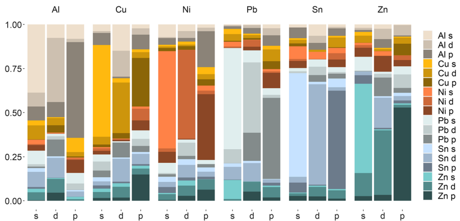
Fig. 1 Aggregated GFEVD plots for weight matrix supply (S). Scaled and aggregated GFEVD of the GVAR with weight matrix supply by the mean of 1 to 10 steps ahead per attribute, decomposed by the shocks of each endogenous variable
