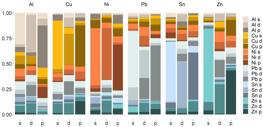
Fig. 3 Aggregated GFEVD plots for weight matrix trading ( T ). Scaled and aggregated GFEVD of the GVAR with weight matrix trading by the mean of 1 to 10 steps ahead per attribute, decomposed by the shocks of each endogenous variable
