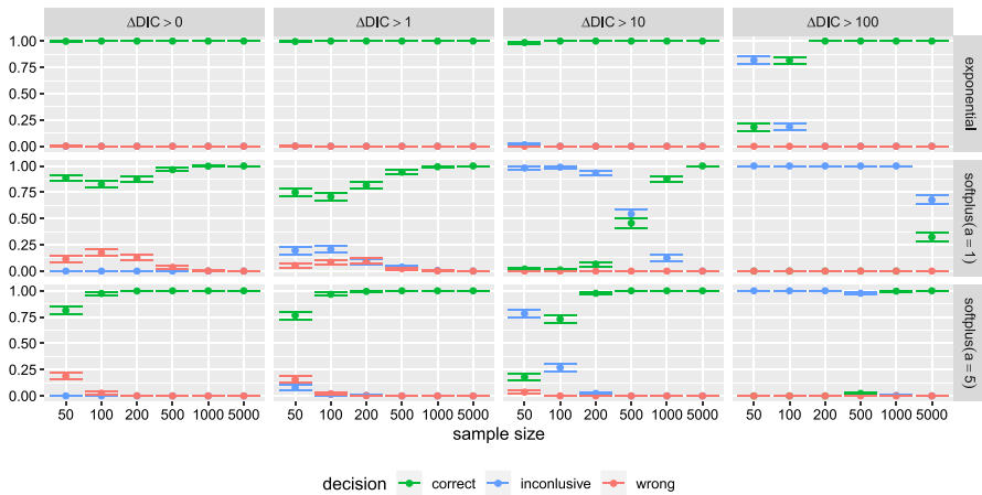
Fig. 4 Percentages of correct model selections based on DIC differences with thresholds 0, 1, 10 and 100 when data are generated with the exponential response function (top row) and the softplus response function (second and third row)
