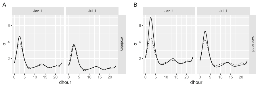
Fig. 8 Predicted standard deviation over the course of a day. Exemplary for the first day of the year 2016 and July 1st on a working day (Panel A) and on a weekend (Panel B). The solid line refers to predictions for the model with exponential response function while the dashed line refers to the model with softplus response function
