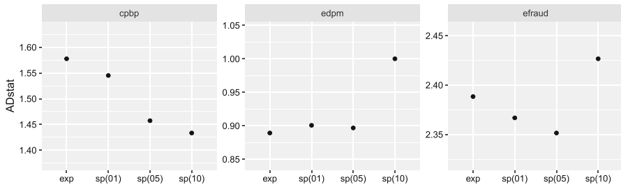
Fig. 13 Anderson-Darling statistics obtained from the RQRs for the three categories
