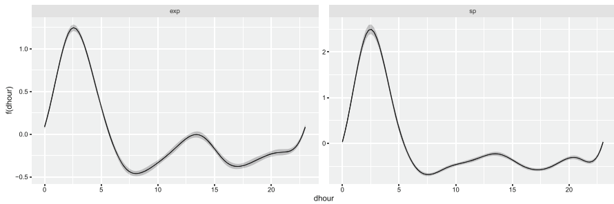
Fig. 7 Posterior mean estimates on the predictor of the standard deviation together with 95% point-wise credible intervals (equal-tailed) for both response functions
