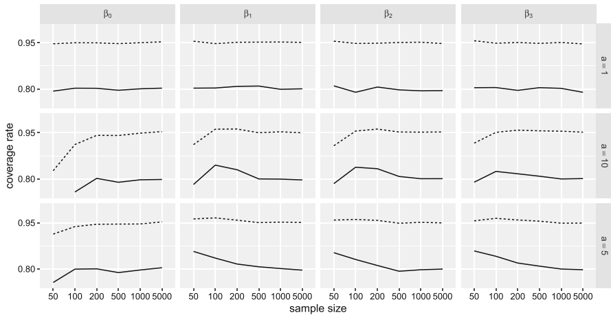
Fig. 3 Coverage probability for 80% (solid line) 95% (dotted line) credible intervals for different sample sizes and different softplus parameters a
