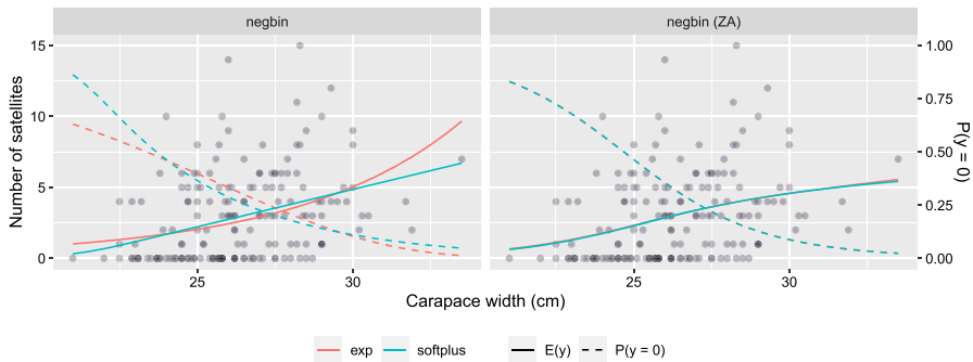
Fig. 5 Plots of the expected response given carapace width and mean color for different response distributions broken down by response function. ZA indicates the the zero-adjusted response distribution. In addition, the dashed line indicates the probability of 0 satellites. The points show the observed data
