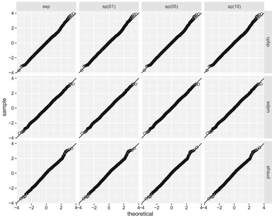
Fig. 10 QQ-plots of the RQRs for the different models. The number in parentheses refers to the employed goodness of approximation parameter in the softplus function
