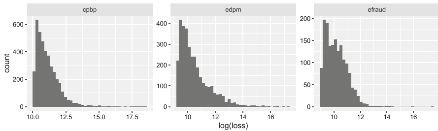
Fig. 9 Histograms of the log-losses larger than the 75% quantile per category, for the three event types
