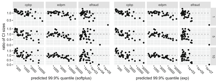
Fig. 12 Ratio of the sizes of the confidence intervals (sp / exp). Left panel: ratio expressed as a function of the softplus posterior mean estimate. Right panel: ratio expressed as a function of the exponential posterior mean estimate. Each row displays the results with the softplus parameter set to the value indicated on the right ( a = 1, 5, 10 )
