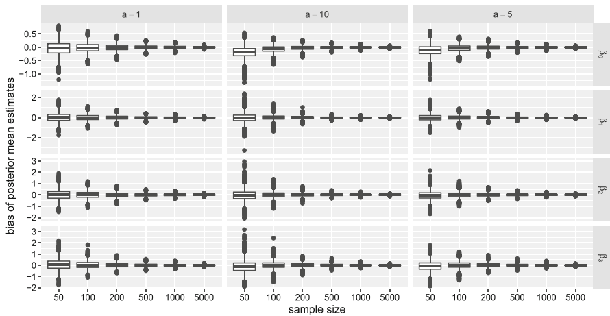
Fig. 2 Box plots of deviations from posterior mean estimates of regression coefficients to the true value for different sample sizes and different softplus parameters a . Replications that include an absolute deviation larger than five for one coefficient have been excluded from plotting for better visualization. This applies to one replication with a = 5 and to ten replications with a = 10 each with a sample size of 50
