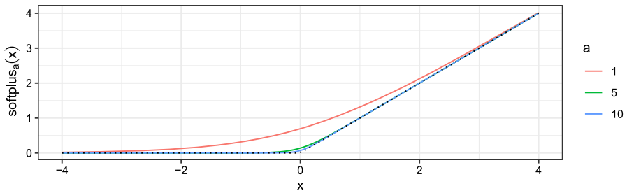
Fig. 1 Plot of the softplus function (left) for different values of softplus parameters a . The approximated linear spline is shown as the dotted line
