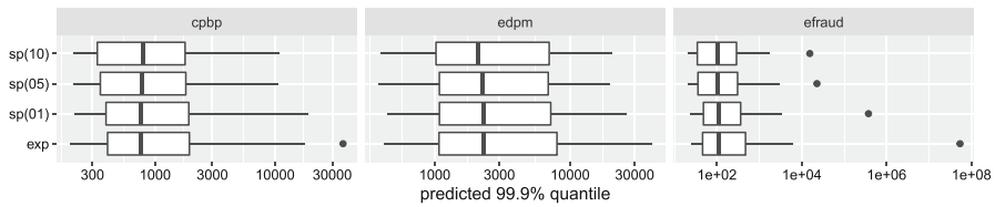
Fig. 11 Box plots of the estimated 99.9% quantiles of the conditional loss size distribution (x-axis is in log-scale).
