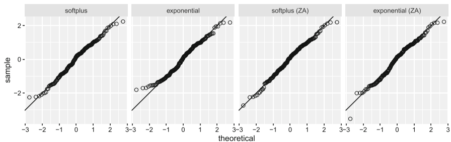
Fig. 6 QQ-plots of one realization of RQRs for negative binomial distributed responses without and with zero-adjustment (indicated by ZA) employing the softplus or the exponential response function
